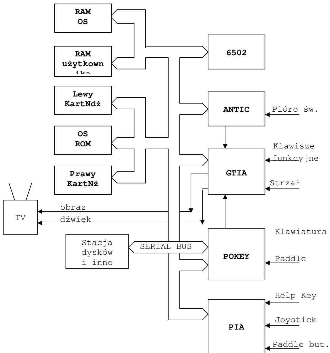
Rys. 1-2 System Atari 400/800
